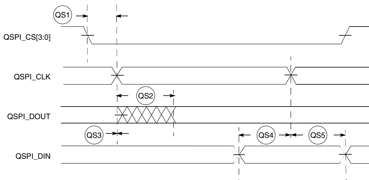
Figure 23-24. QSPI Timing
