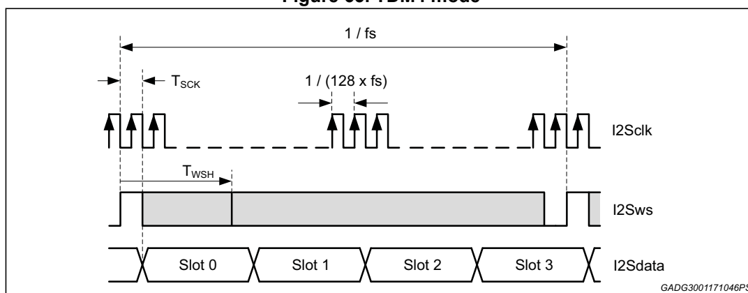
Figure 65. TDM4 mode
