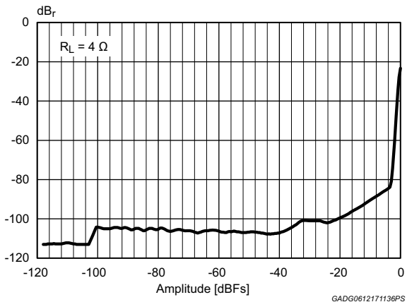
Figure 36. Dynamic range
