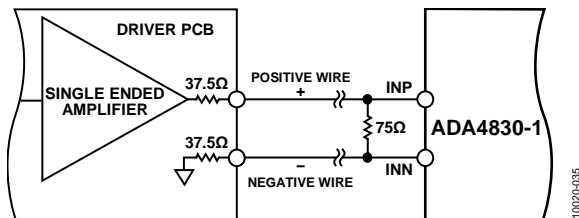
Figure 22. Pseudo Differential Mode with Balanced Source Impedance
