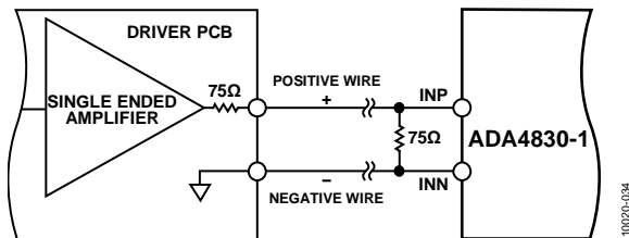
Figure 21. Pseudo Differential Mode
