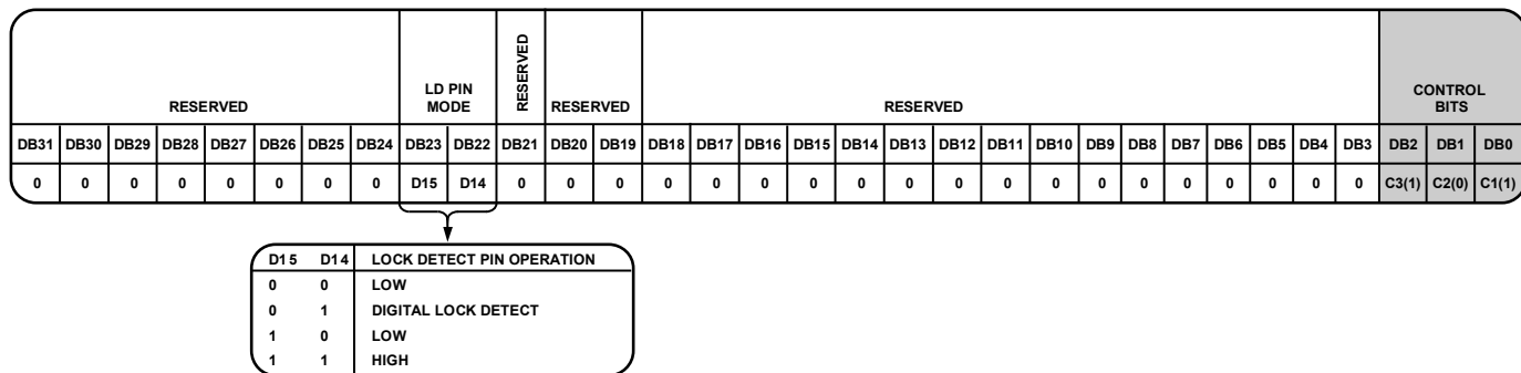
Figure 29. Register 5 (R5)
