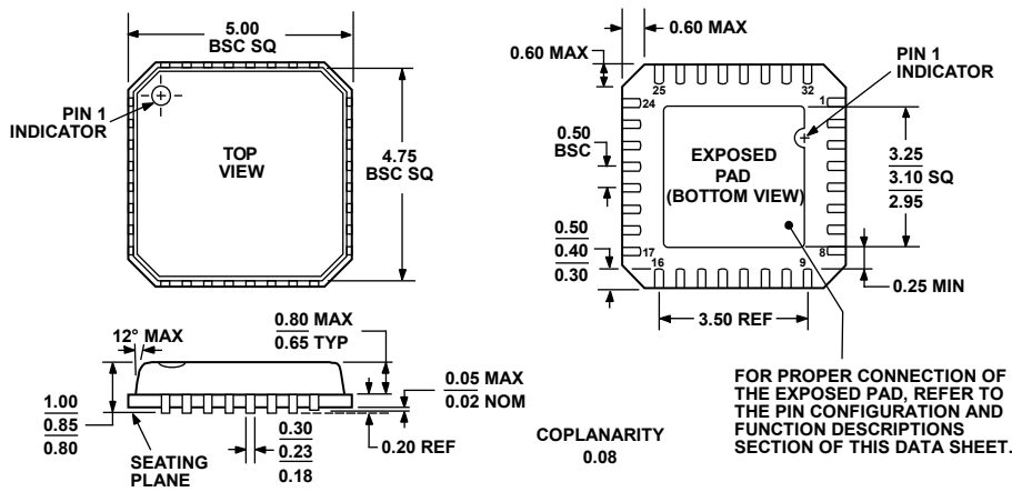
COMPLIANT TO JEDEC STANDARDS MO-220-VHHD-2 Figure 40. 32-Lead Lead Frame Chip Scale Package [LFCSP_VQ] 5 mm × 5 mm Body, Very Thin Quad (CP-32-2) Dimensions shown in millimeters
