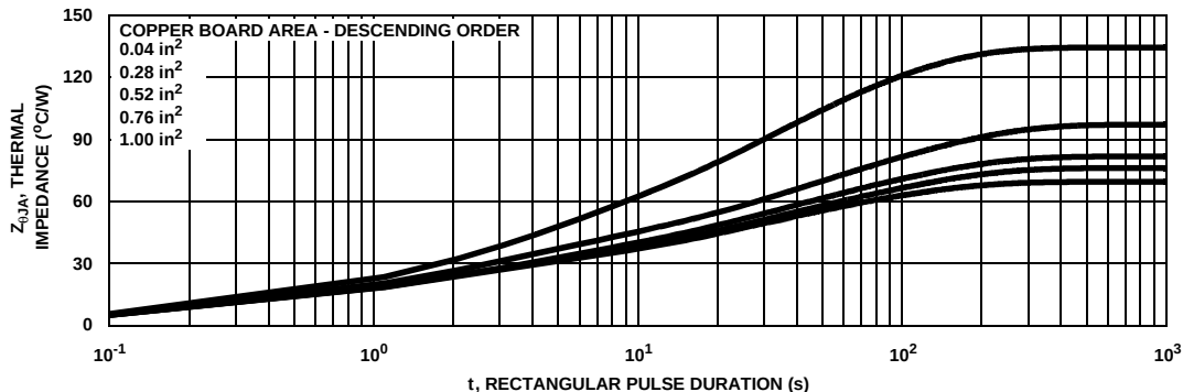
Figure 20. Thermal Impedance vs Mounting Pad Area
