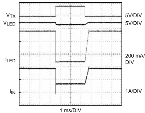
Figure 32. Tx-Mask Event
