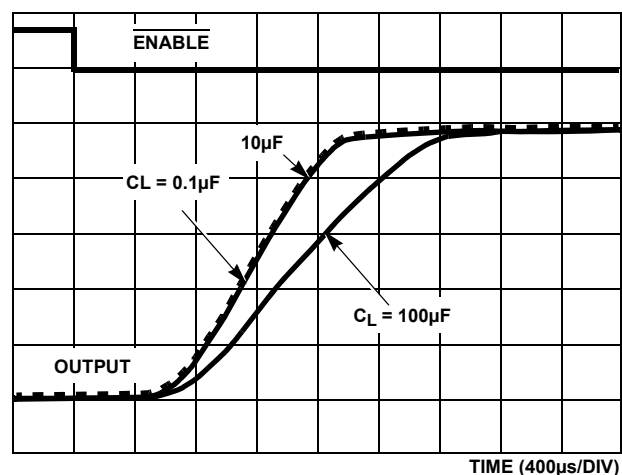
FIGURE 3. VOUT SOFT START vs C_{LOAD} , R_I = 10\Omega
