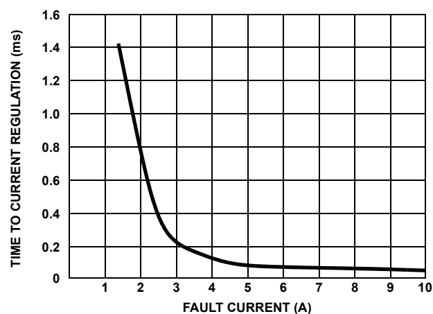
FIGURE 7. CR SETTLING TIME vs FAULT CURRENT
