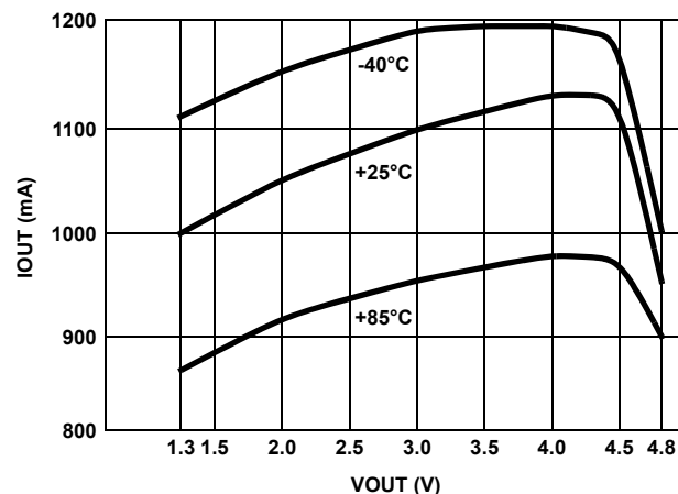
FIGURE 5. CURRENT REGULATION vs VOUT (VIN = 5.0V)
