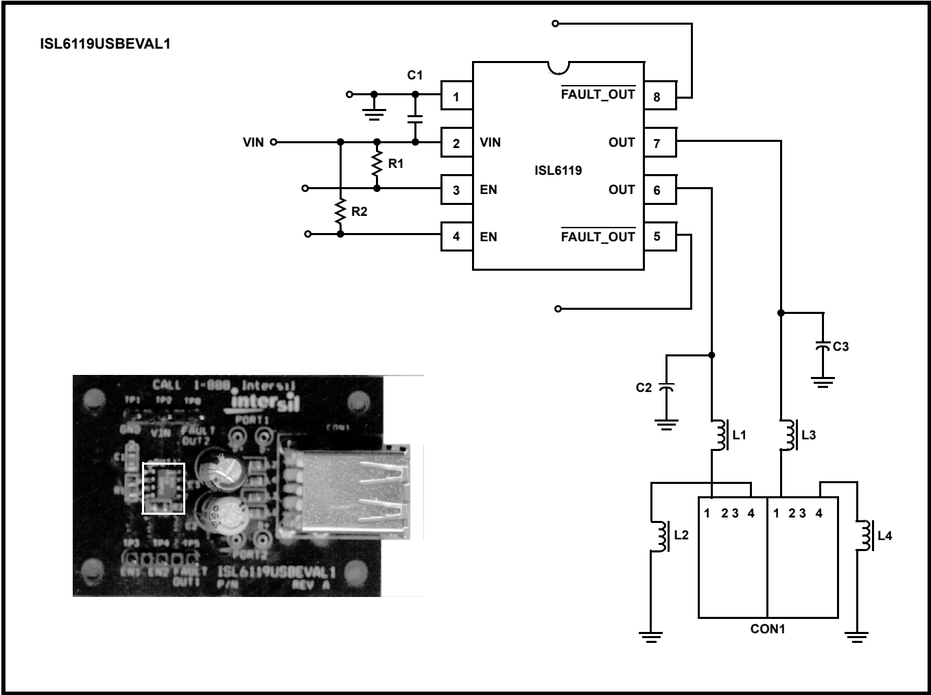
FIGURE 20. ISL6119USBEVAL BOARD
