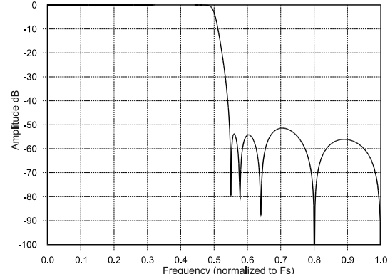
Figure 39. DAC Stopband
