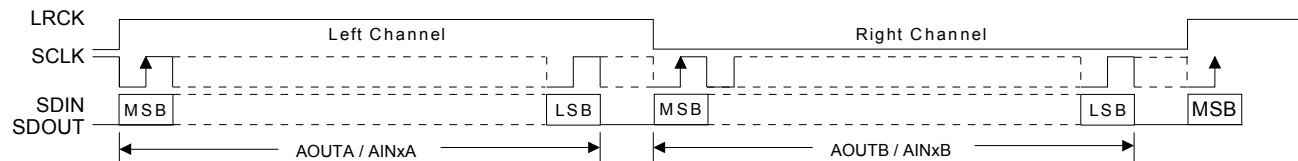
Figure 20. Left-Justified Format
