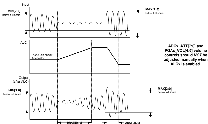
Figure 11. ALC
