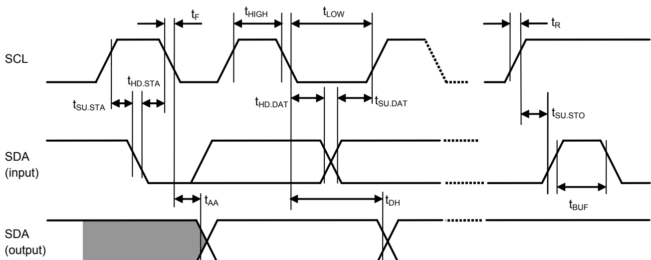
Figure 8 Bus Timing
