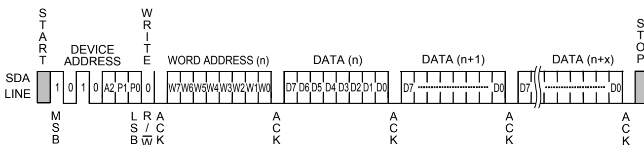
Figure 16 Page Write
