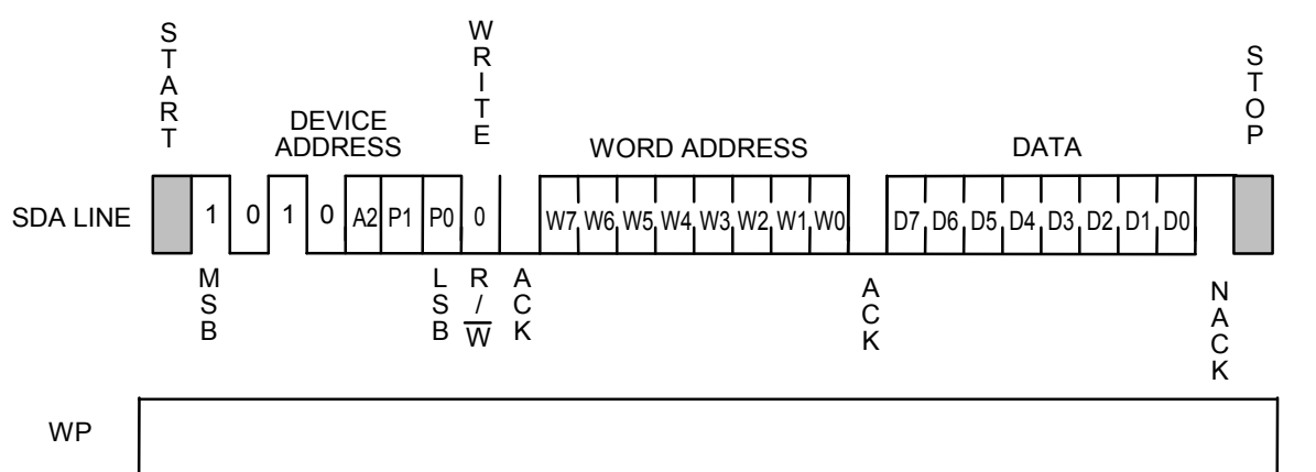
Figure 17 Write Protect
