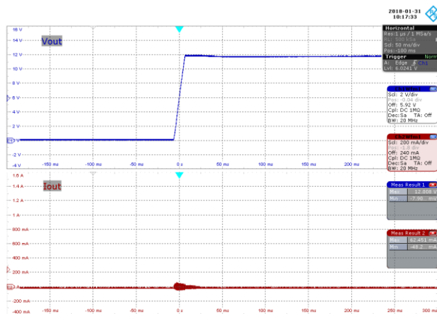
Figure 51 – 265 VAC 60 Hz, No-Load Start-up.
