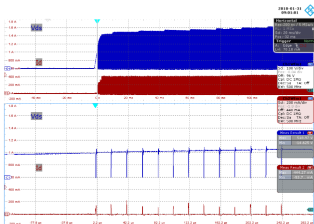
Figure 70 – 230 VAC 60 Hz, Full Load Start-up.
