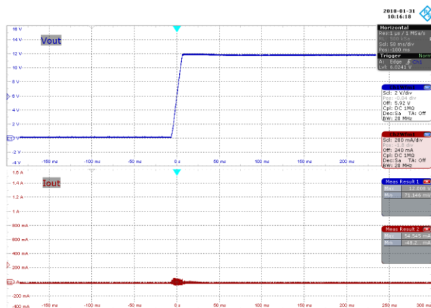
Figure 49 – 115 VAC 60 Hz, No-Load Start-up.
