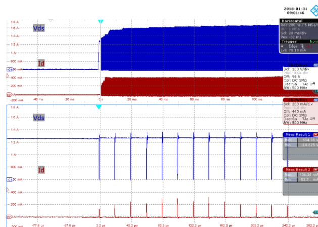
Figure 71 – 265 VAC 60 Hz, Full Load Start-up.
