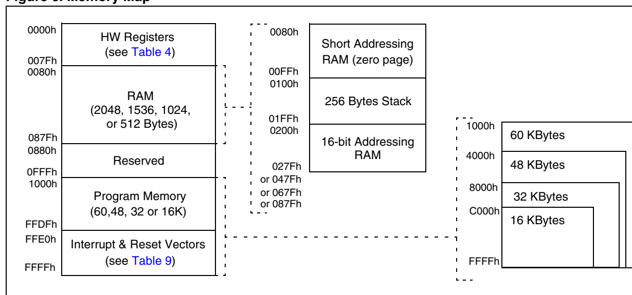
Figure 6. Memory Map
