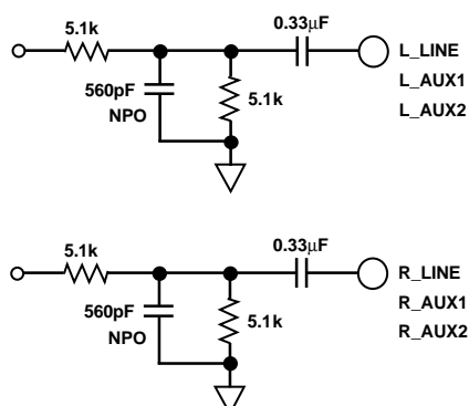
Figure 17. AD1848K 2 V rms Line-Level Input Circuit
