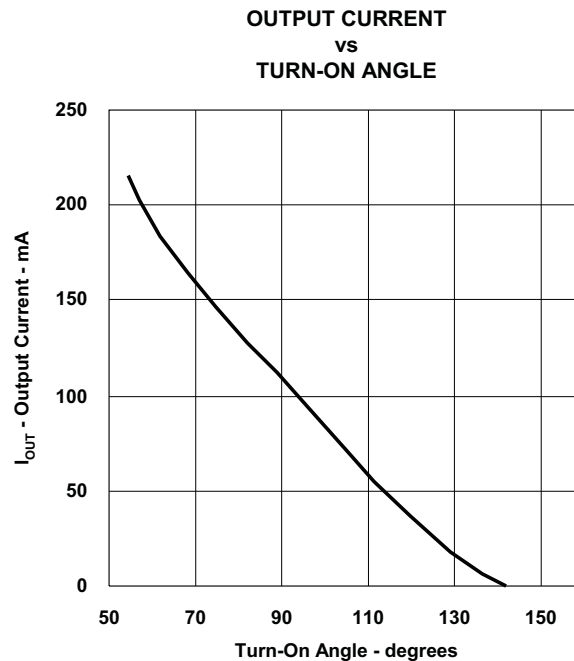
Figure 9. TRIAC Dimmer Performance
