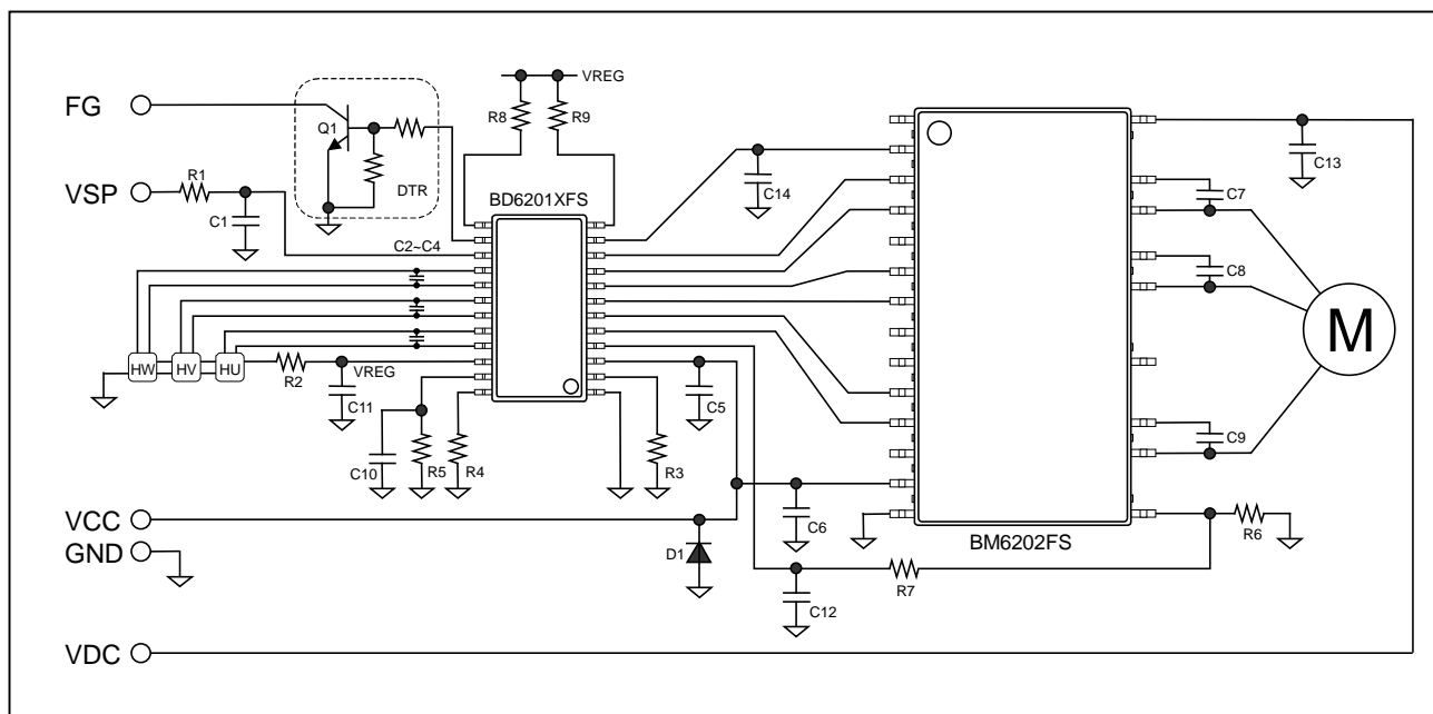
Figure 1. Application circuit example - BM6202FS &amp; BD6201XFS
