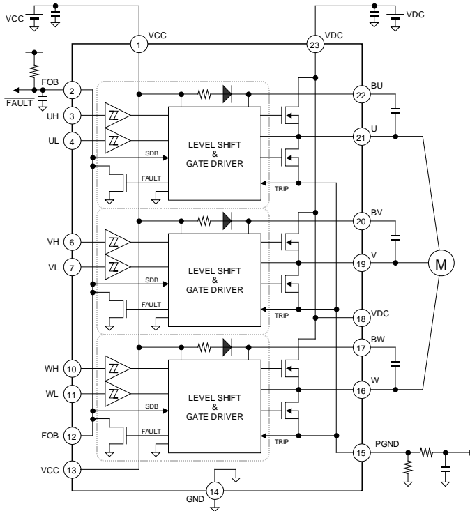
Figure 2. Block diagram
