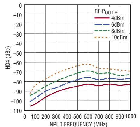
HD4 vs Input Frequency Over P_{\text{OUT}}
