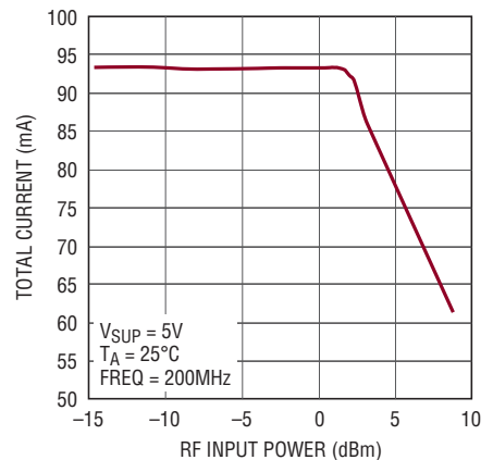
Total Current vs RF Input Power
