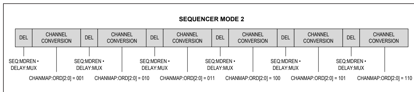
Figure 7. Sequencer Mode 2 Timing Diagram
