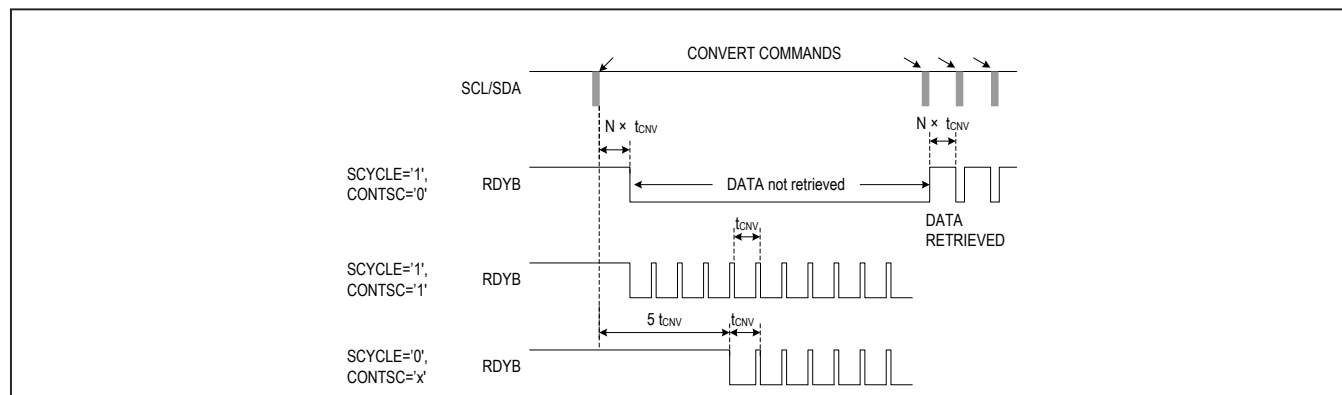
Figure 4. Timing of RDYB in All Conversion Configurations: Single-Cycle, Single-Cycle Continuous and Continuous. In sequencer mode 1 and in sequencer modes 2 and 3, with SEQ:RDYBEN='0' N = 1. In sequencer modes 2 and 3 with SEQ:RDYBEN='1' N = number of active channels.
