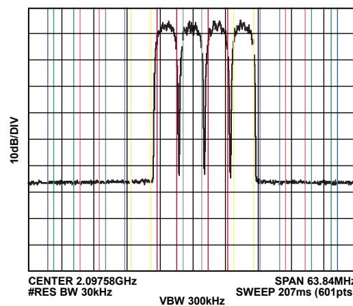
Figure 31. Typical Single-Carrier WCDMA ACLR Performance at 2.8 GHz, f_{DAC} = 2457.6 MSPS (Third Nyquist Zone)
