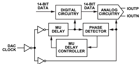
Figure 48. Mu Delay Controller Block Diagram
