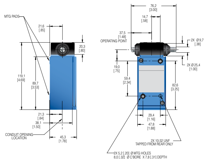
DPDT Non-plug-in (mm[in])
