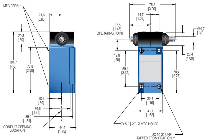
SPDT Non-plug-in (mm[in])
