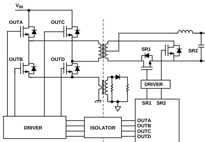
Figure 21. PWM Pin Assignment for Full-Bridge, Phase-Shifted Topology with Synchronous Rectification
