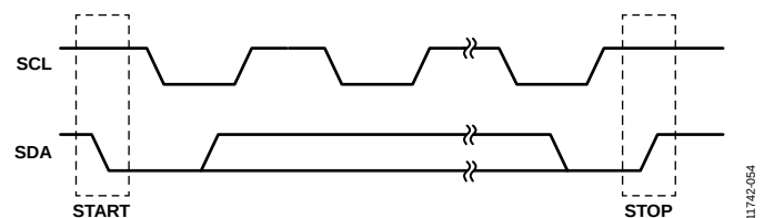
Figure 54. Start and Stop Transitions
