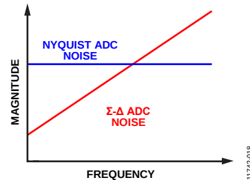
Figure 18. Noise Performance for Nyquist Rate and \Sigma\text{-}\Delta ADCs
