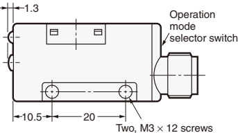
Mounting Holes
