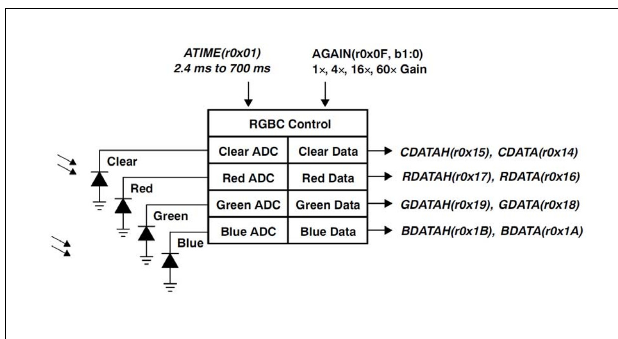
Figure 23: RGBC Operation
