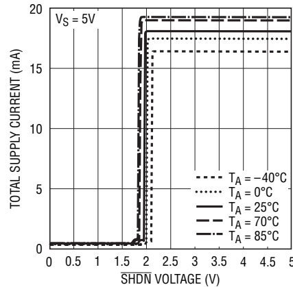
Supply Current vs \overline{\text{SHDN}} Voltage
