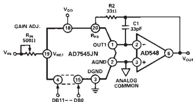
Figure 4. AD548 Used as DAC Output Amplifier
