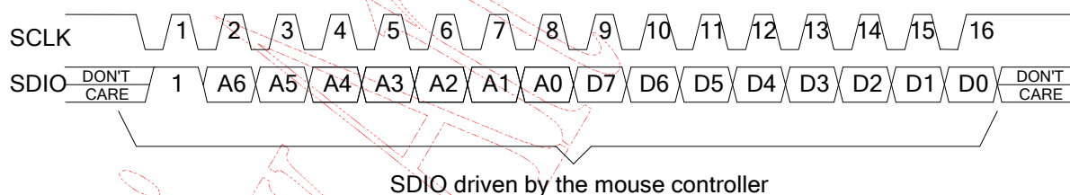
Figure 8. Write Operation
