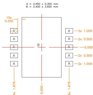
PCB Metal Land Pattern
