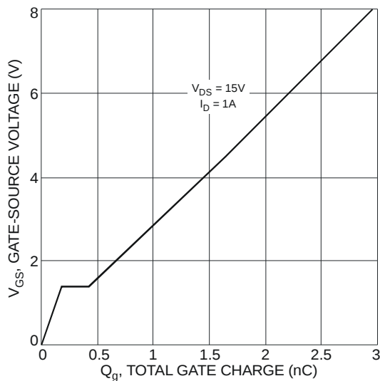
Fig. 14 Gate-Charge Characteristics
