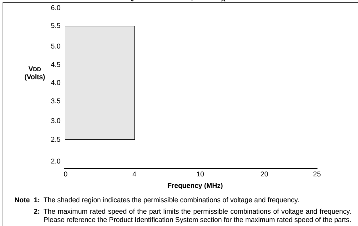
FIGURE 10-3: VOLTAGE-FREQUENCY GRAPH, 0^{\circ}\text{C} \leq T_A \leq +85^{\circ}\text{C}
