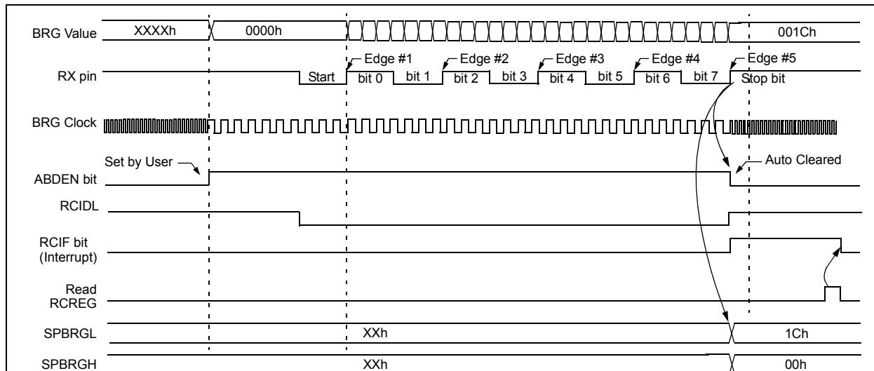
FIGURE 23-6: AUTOMATIC BAUD RATE CALIBRATION
