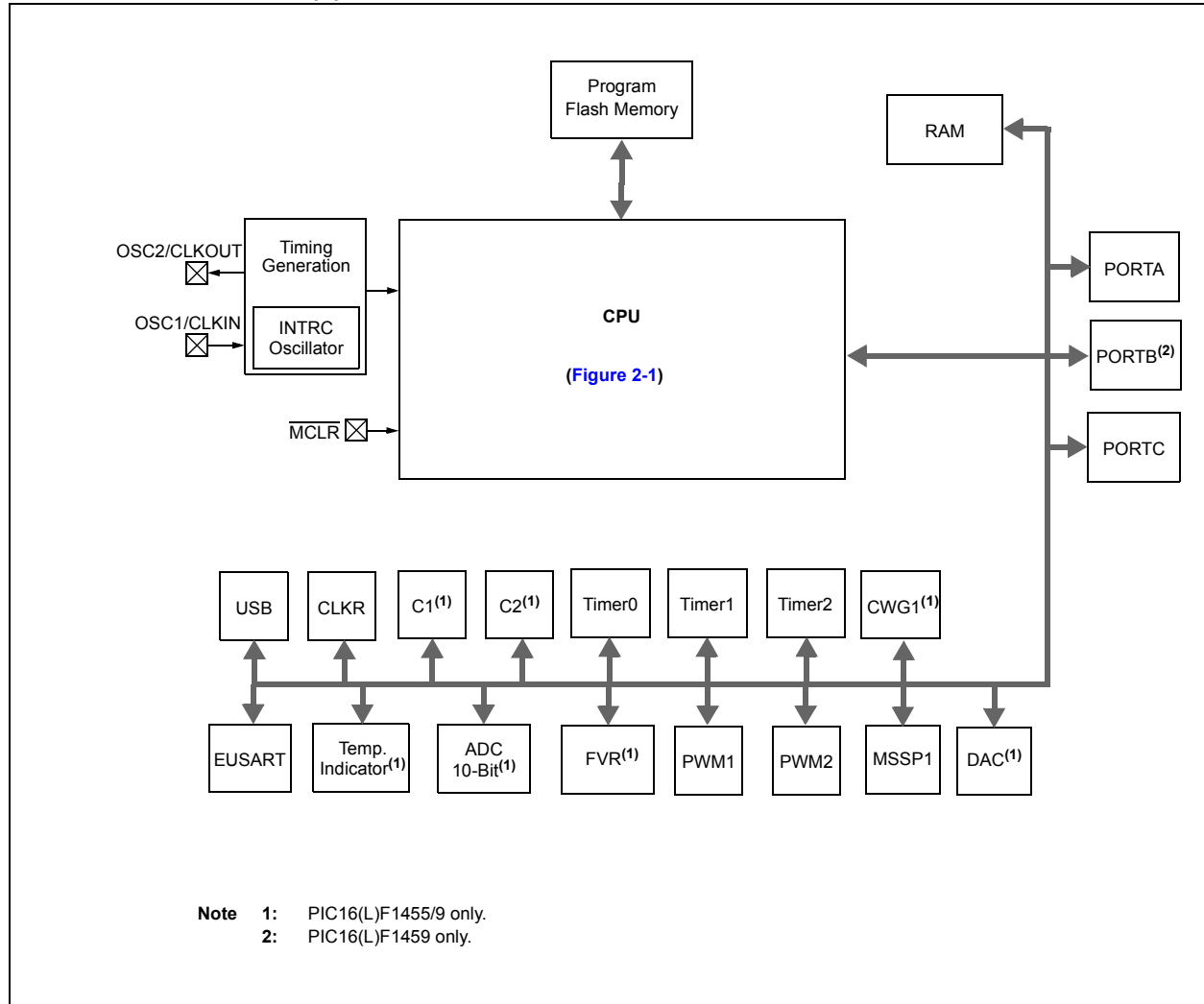
FIGURE 1-1: PIC16(L)F1454/5/9 BLOCK DIAGRAM
