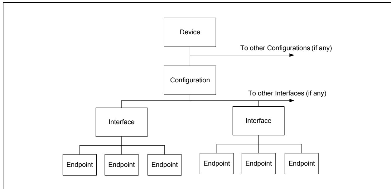
FIGURE 26-11: USB LAYERS
