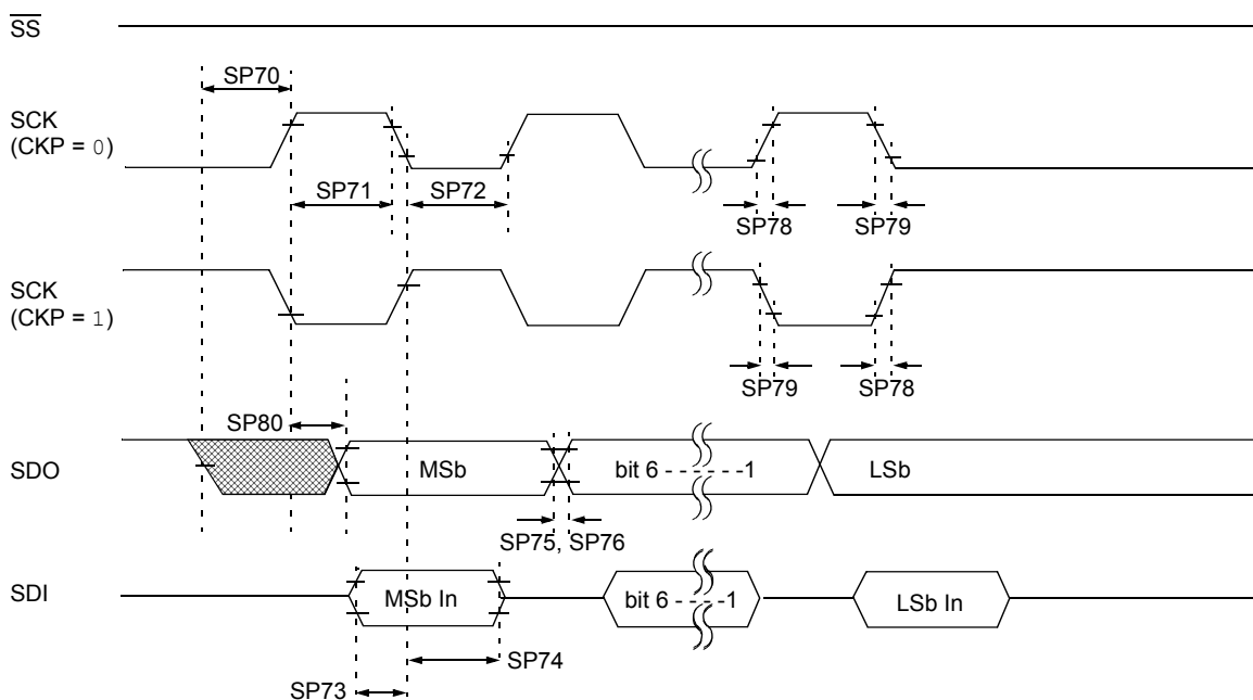
FIGURE 29-14: SPI MASTER MODE TIMING (CKE = 0, SMP = 0)
