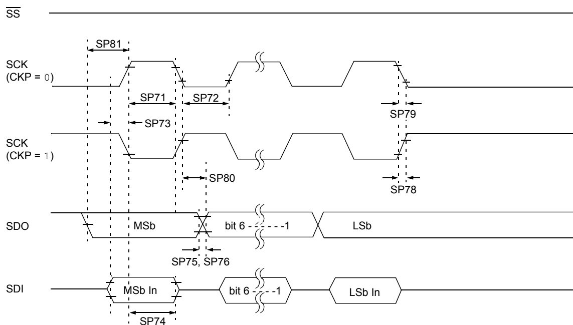
FIGURE 29-15: SPI MASTER MODE TIMING (CKE = 1, SMP = 1)
