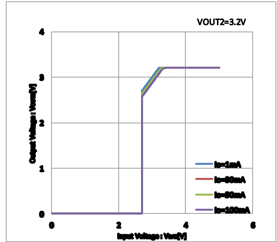
Figure 13. Output Voltage VS Input Voltage (VBAT=0V~5.5V,Ta=25°C,Vout=3.2V)
