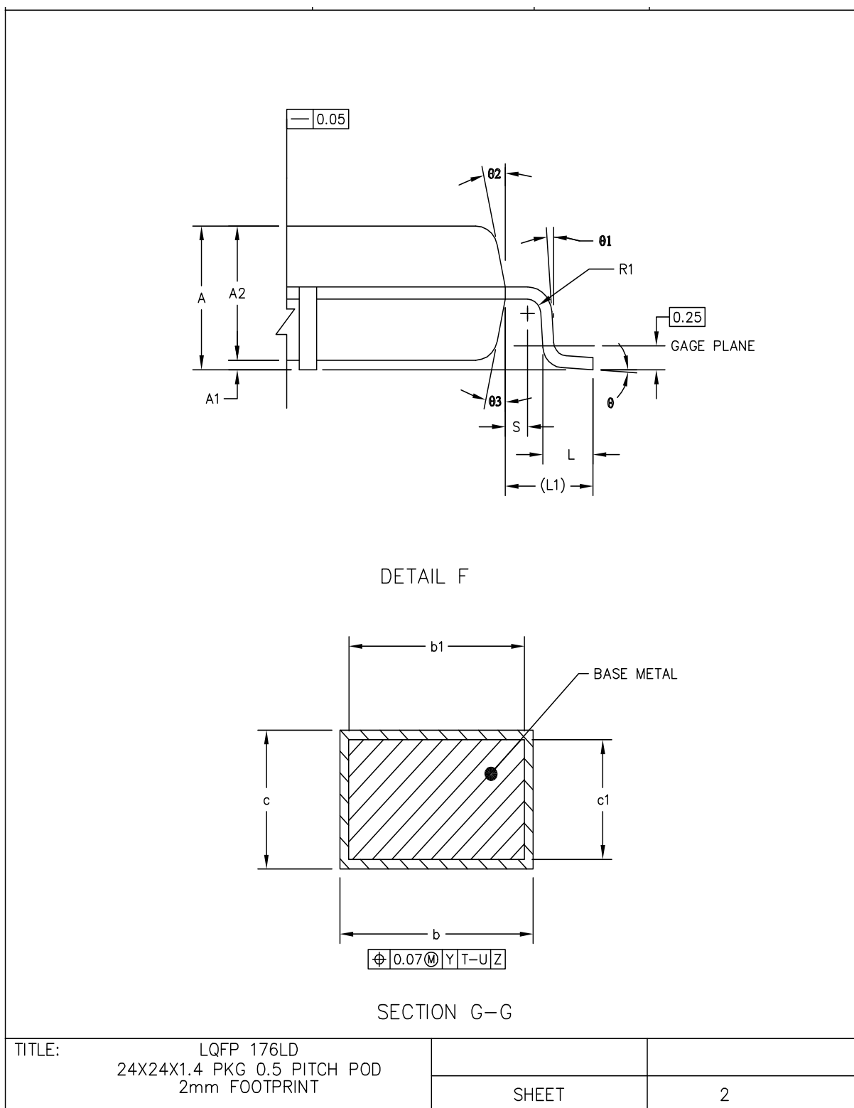
Figure 38. 176 LQFP mechanical drawing (Part 2 of 3)
