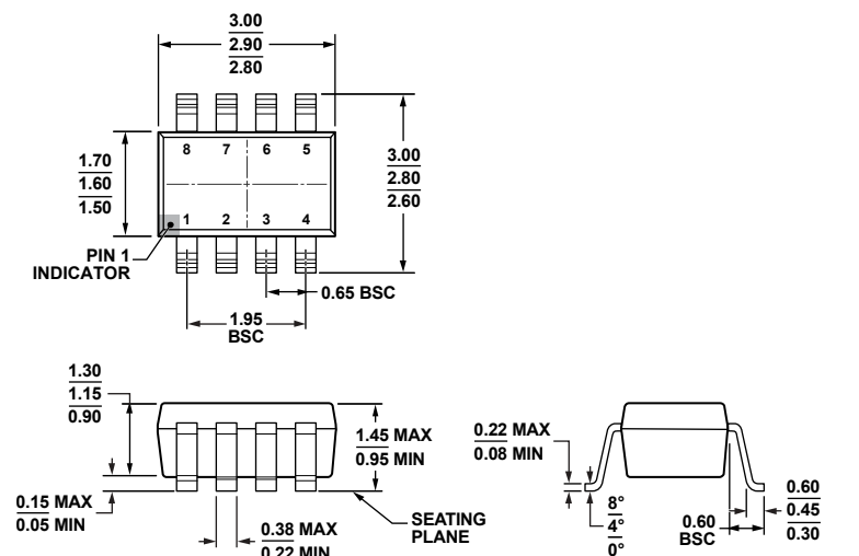
COMPLIANT TO JEDEC STANDARDS MO-178-BA Figure 38. 8-Lead Small Outline Transistor Package [SOT-23] (RJ-8)
