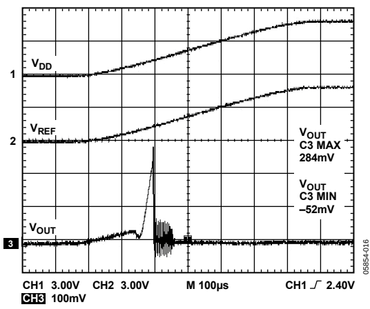
Figure 15. Power-On Reset to 0 V
