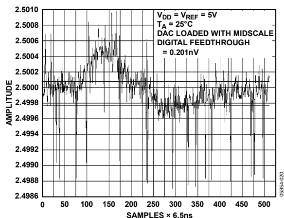
Figure 18. Digital Feedthrough
