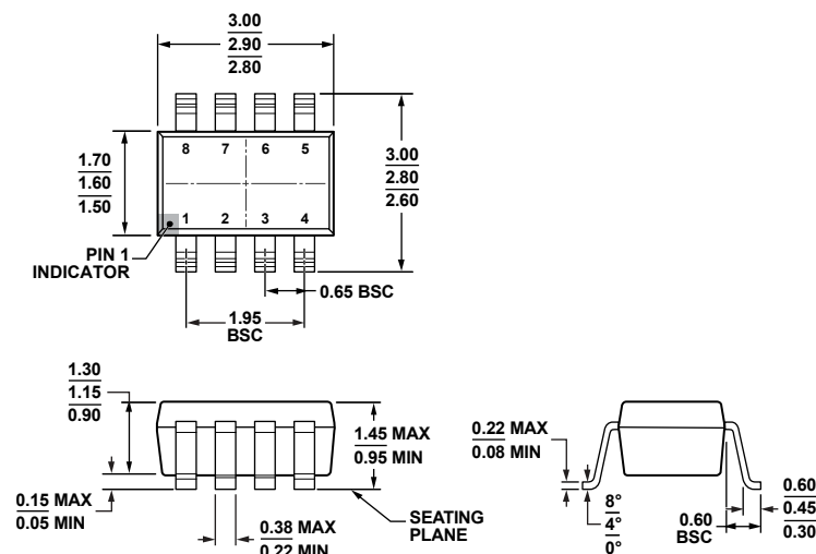
COMPLIANT TO JEDEC STANDARDS MO-178-BA Figure 38. 8-Lead Small Outline Transistor Package [SOT-23] (RJ-8)
