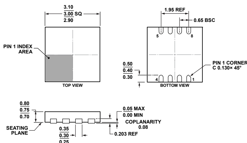
COMPLIANT TO JEDEC STANDARDS MO-229-WEEC-2 Figure 39. 8-Lead Lead Frame Chip Scale Package [LFCSP_WD] 3 mm × 3 mm Body, Very Very Thin, Dual Lead (CP-8-15)
