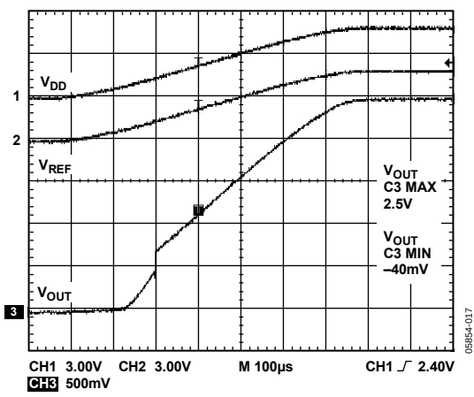
Figure 16. Power-On Reset to Midscale
