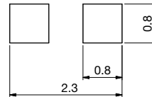
Recommended solder pad footprint
