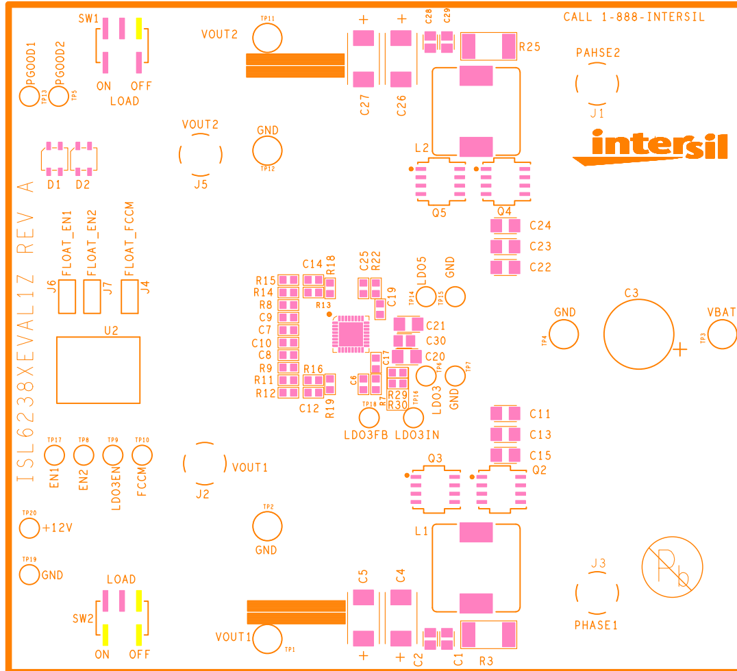
FIGURE 3. TOP SILKSCREEN
