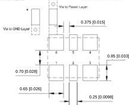
Recommended Solder Pad Layout units: mm[inch]
