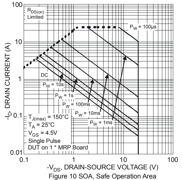
Figure 10 SOA, Safe Operation Area
