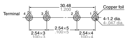
Mounting hole location (Bottom view)
