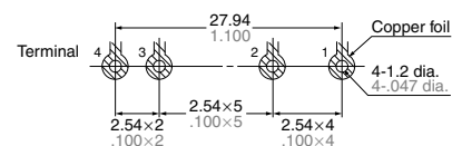
Mounting hole location (Bottom view)
