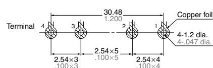
Mounting hole location (Bottom view)
