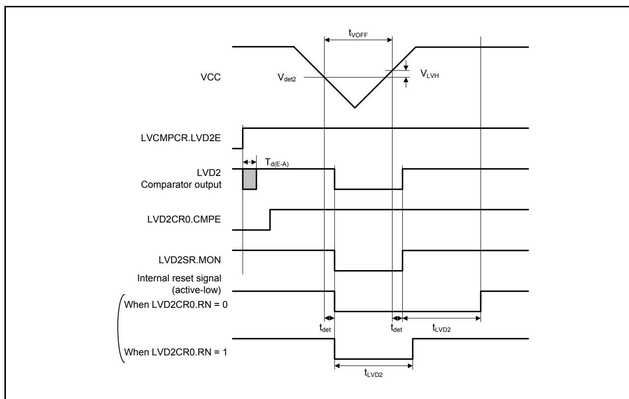
Figure 2.70 Voltage detection circuit timing ( V_{\text{det2}} )
