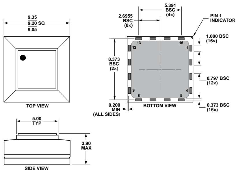
Figure 36. 16-Terminal Land Grid Array [LGA] (CC-16-2) Dimensions shown in millimeters
