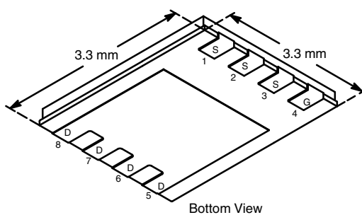
PowerPAK® 1212-8
