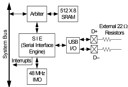
Figure 7-16. USB
