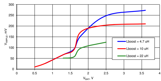
Figure 11-14. V_{RIPPLE} vs V_{BAT} [42]
