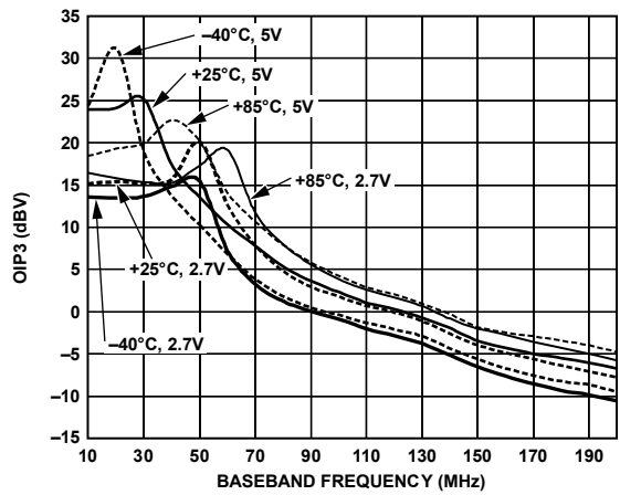
Figure 35. OIP3 vs. F_{BB} , V_{VCMO} = V_{REF} = 1 V , V_{POS} = 2.7 V, 5 V , Temperature = -40^{\circ}C, +25^{\circ}C, +85^{\circ}C
