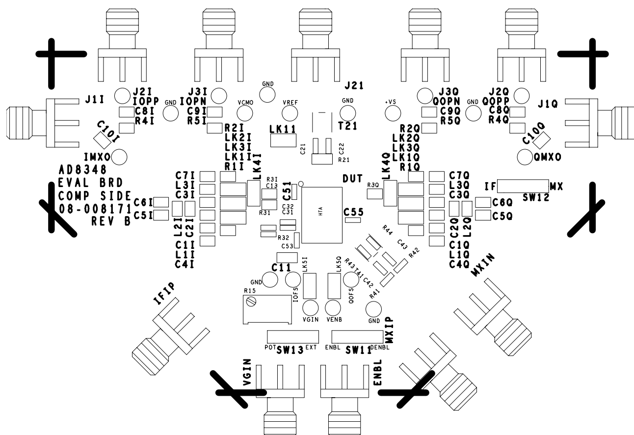
Figure 62. Evaluation Board Top Silkscreen
