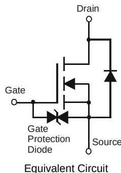
Equivalent Circuit
