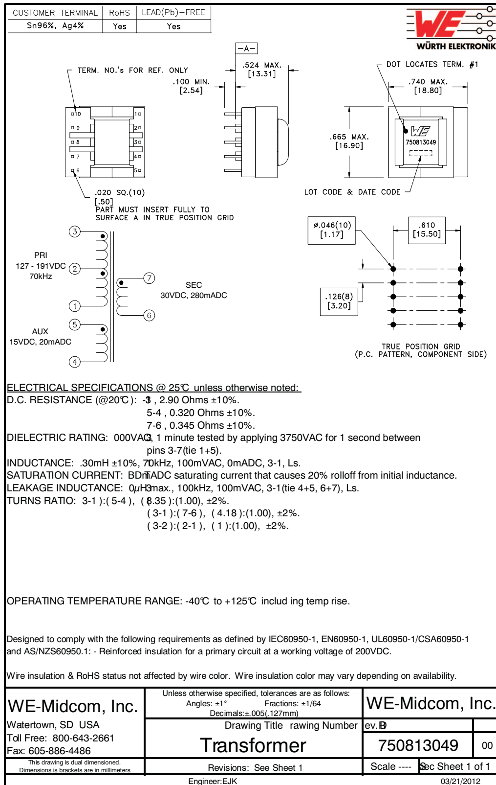
Figure 28. Transformer Specification
