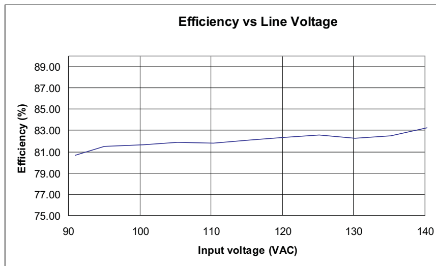
Figure 3. LM3447-A19-120VEVM Efficiency
