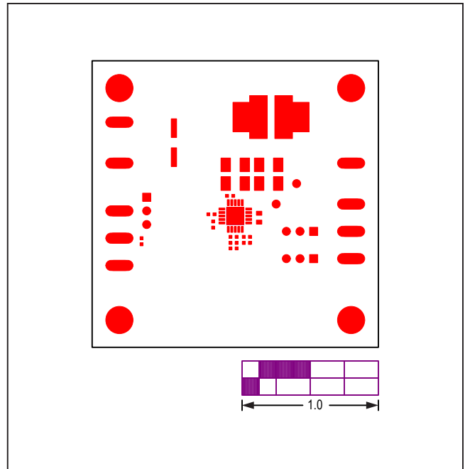
Figure 17. MAX17544 3.3V Output EV Kit Component Placement Guide—Top Solder Mask
